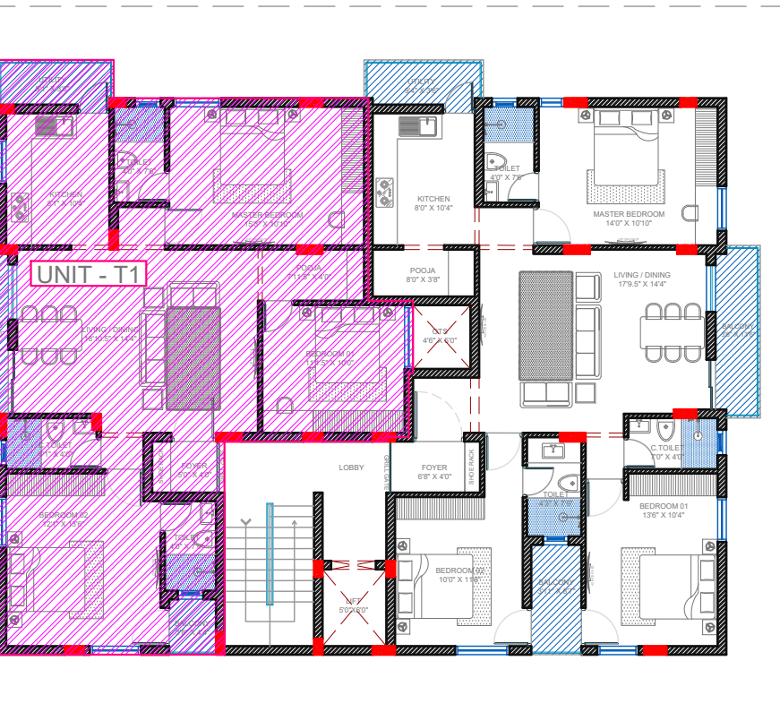
THIRD FLOOR KEY PLAN - UNIT T1
