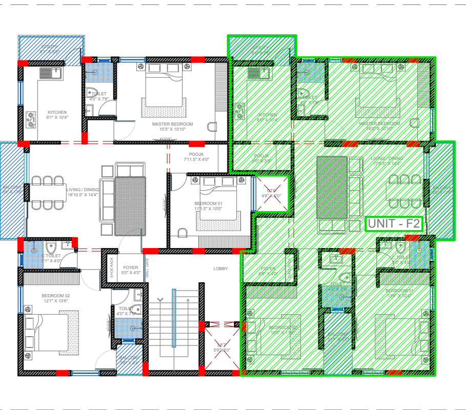
FIRST FLOOR KEY PLAN - UNIT F2
