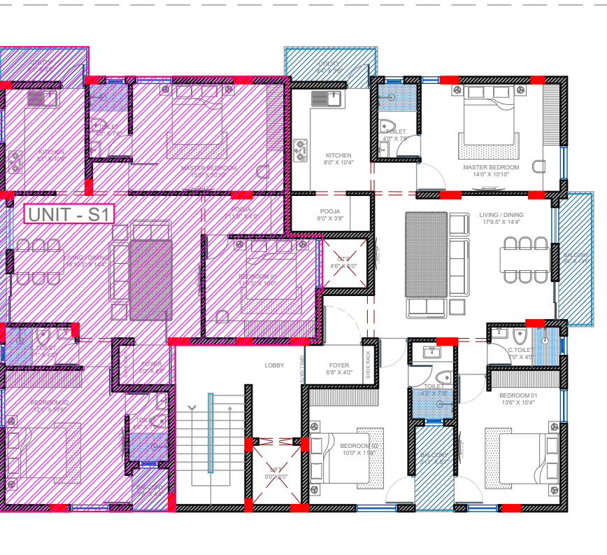
SECOND FLOOR KEY PLAN - UNIT S1
